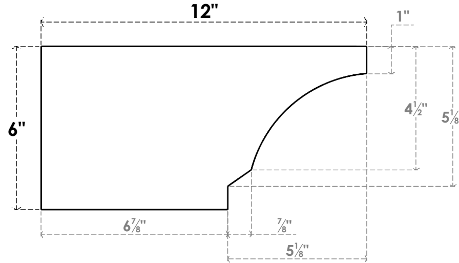
SIDE PROFILE
